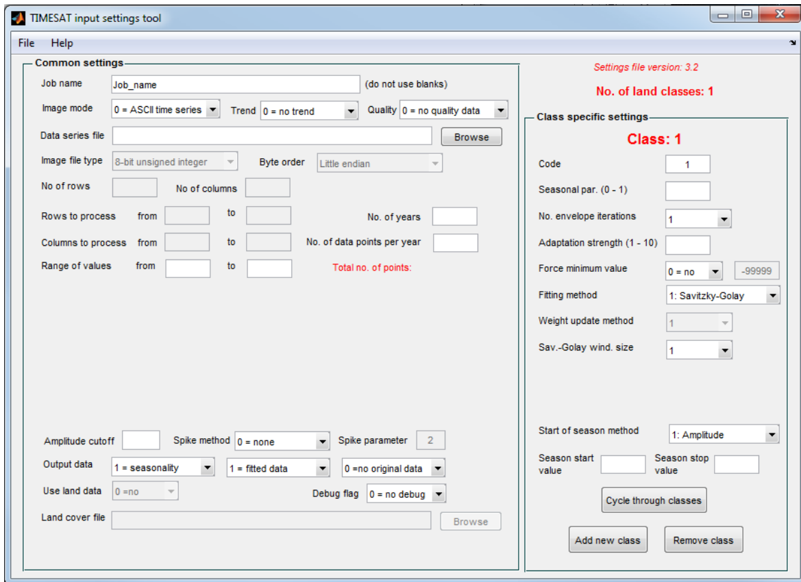
Figure 31: TSM_settings window. Common settings are defined in the left pane and class specific in the right pane.
