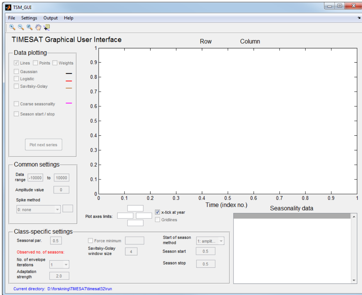
Figure 29: TSM_GUI . This is the main program for fitting functions to time-series data for selected pixel locations or for single ASCII data files.
