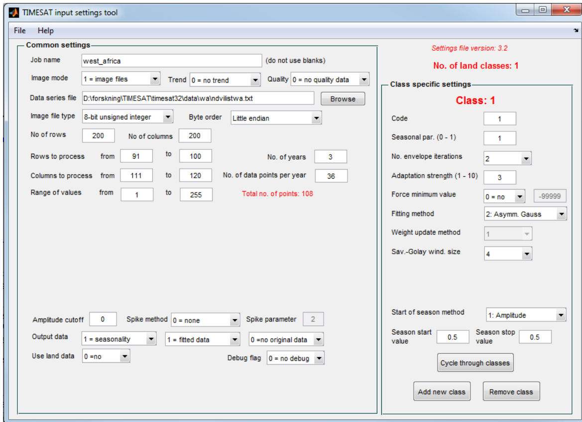
Figure 23: TSM_settings with settings for West Africa. Common settings are shown in the left pane and class specific settings in the right pane. For more information please see text.
