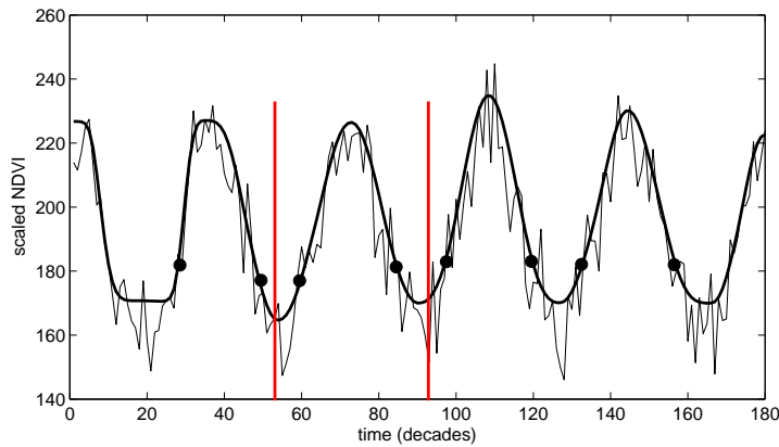
Figure 17: To extract information from the seasonality file for a specific season a time window must be defined. The season for which the start and end of the season lies within the window is the desired one.
