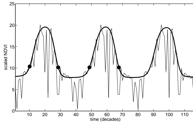
Figure 13: To extract seasonality parameters from one year of data the time-series has been duplicated to span three years.
