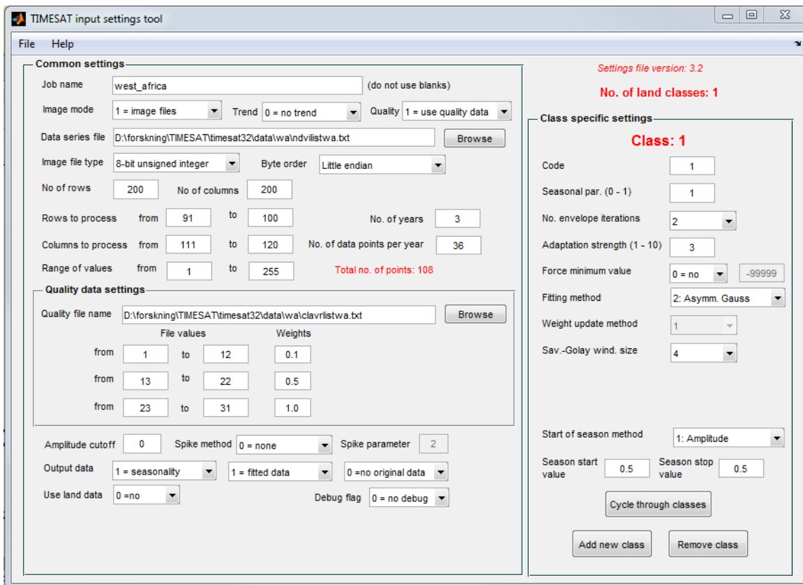
Figure 24: TSM_settings with quality data.
