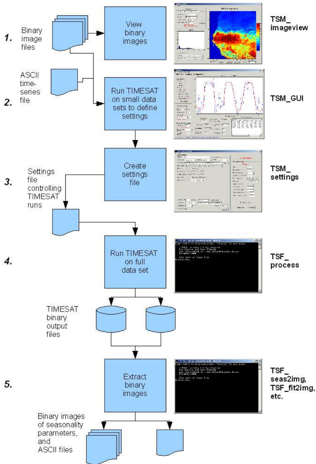
Figure 18: General TIMESAT processing logic. The numbers in the left margin describe the step involved in the data processing. Please refer to the text for further details.
