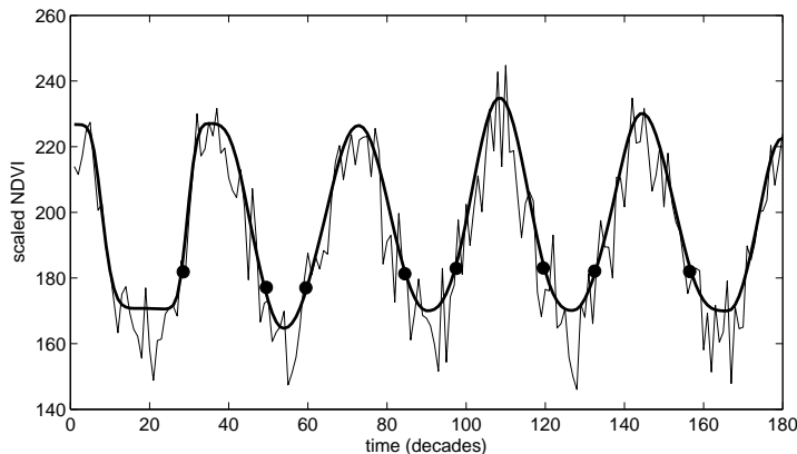
Figure 12: Time-series covering a period of 5 years. Only seasonality parameters from the 4 full seasons can be determined from fitted functions. The start and end of the seasons are marked with filled circles.
