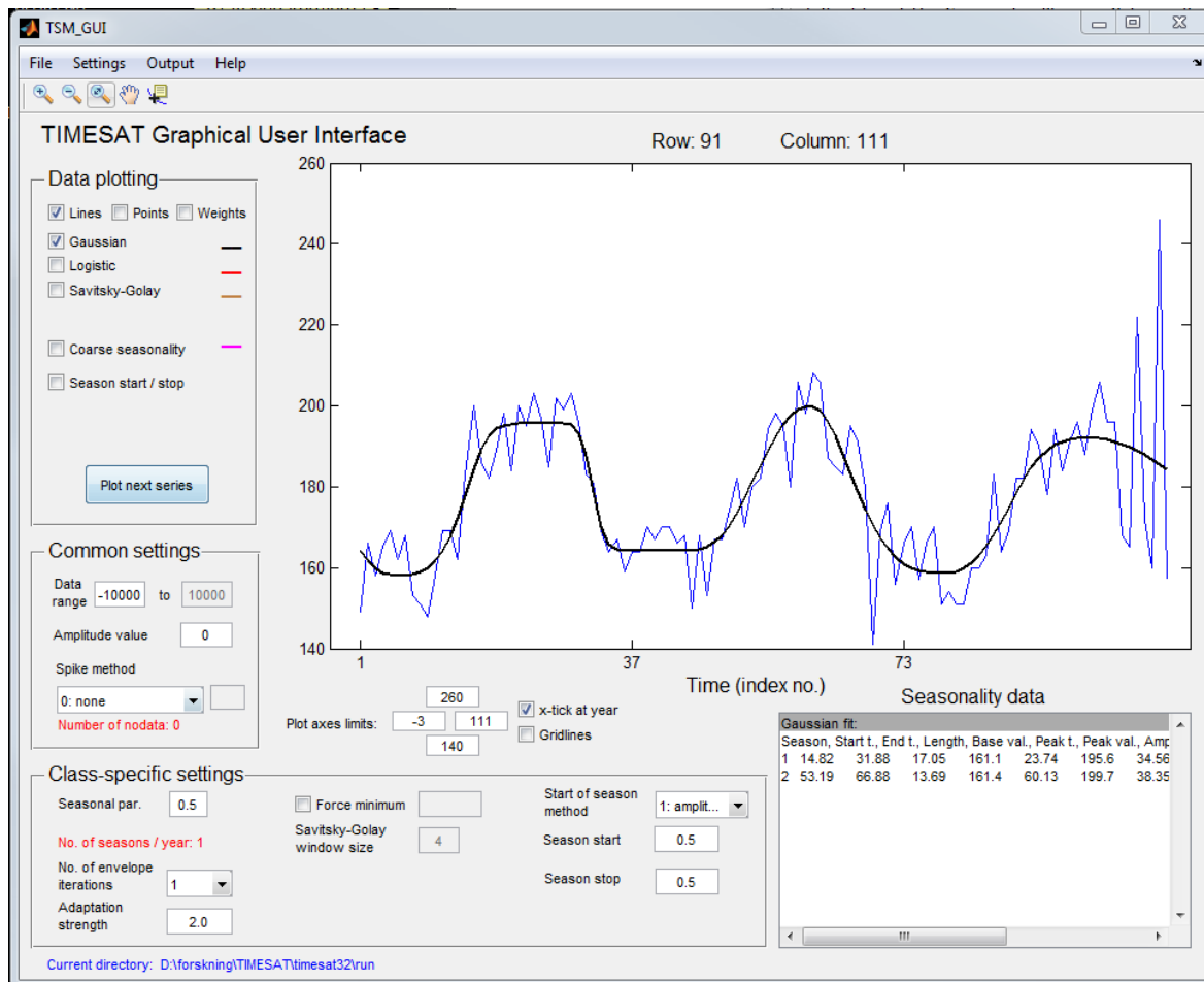
Figure 22: TSM_GUI showing NDVI over West Africa, row 91, column 111. The asymmetric Gaussian model fit is displayed along with the raw data values.
