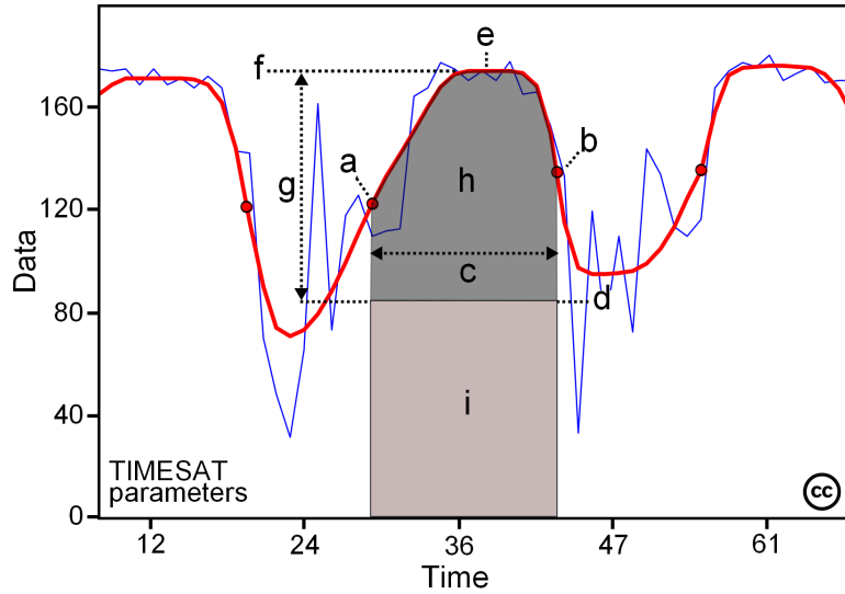
Figure 14: Figure 1. Some of the seasonality parameters generated in TIMESAT: (a) beginning of season, (b) end of season, (c) length of season, (d) base value, (e) time of middle of season, (f) maximum value, (g) amplitude, (h) small integrated value, (h+i) large integrated value. This figure is licensed under a Creative Commons Attribution-NonCommercial-NoDerivs 2.5 Sweden License. It is free to copy and use in other work.
