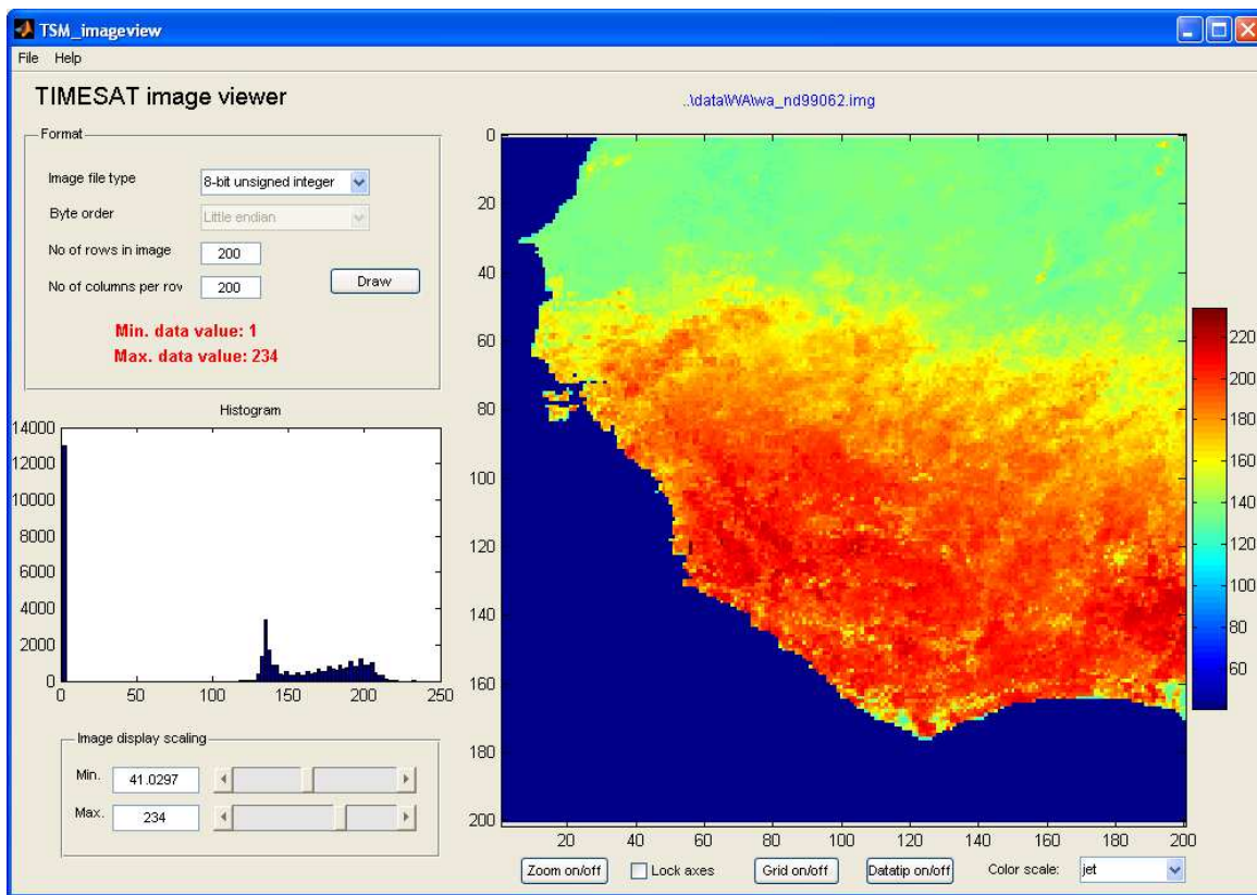
Figure 21: TSM_imageview with a loaded vegetation index image. The program can be used to view binary image data and explore the correct settings for the file format of images.
