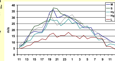
Fig. 3. Gust wind speed measured at SMHI automatic stations during the period December 03 11 UTC — 04 13 UTC. Station letters refer to Fig. 2.
