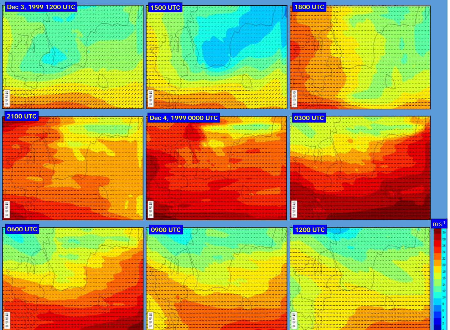
These figures represent a time sequence of the 920 hPa wind vectors and intensity fields simulated with the 2-km CRCM over southern Sweden during the Anatol storm. Vector intensities are shown in insets and intensity in \text{ms}^{-1} by a color scale (right).
